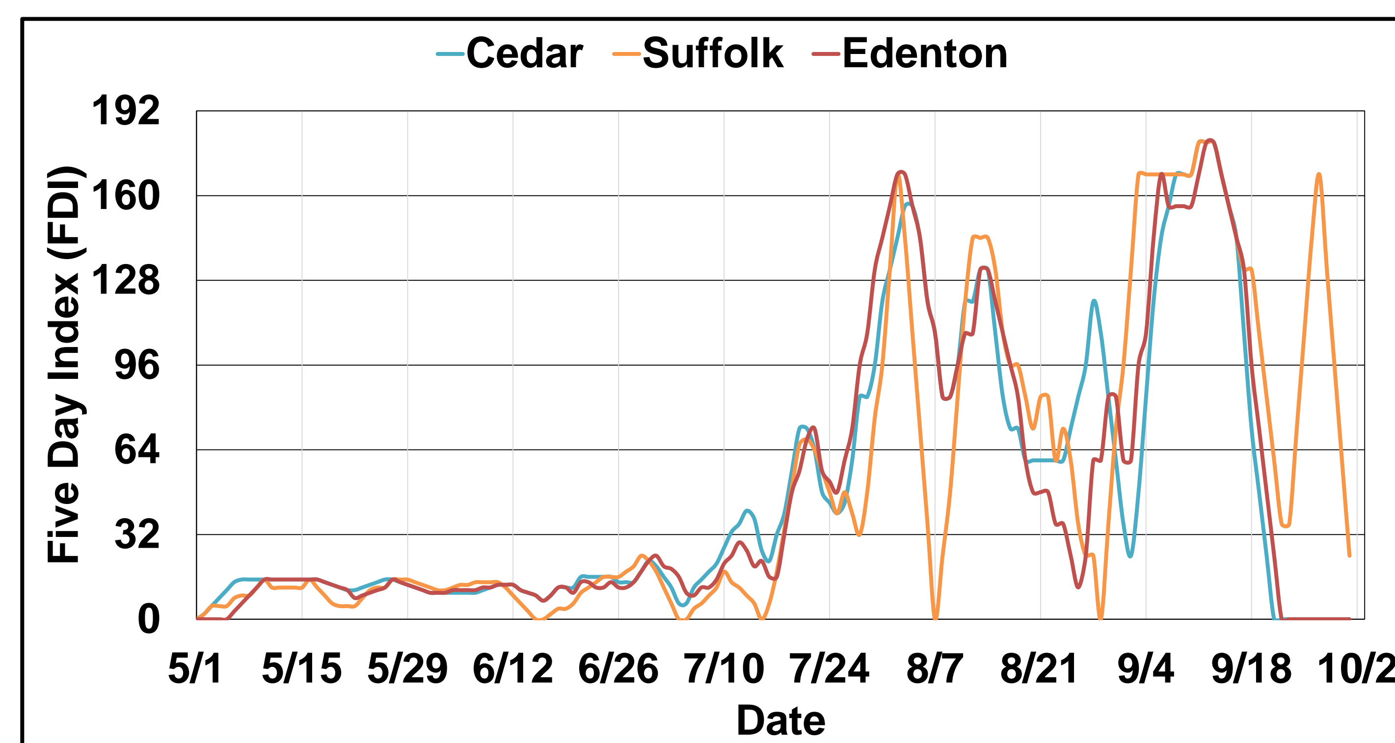
Figure 3. The five day index (FDI) for Sclerotinia blight risk with the current weather-based disease model being used for Virginia peanut advisories. Based on the model, all locations reached threshold (FDI = 32) by July 21, but Sclerotinia was not observed until August (see Table 1).
